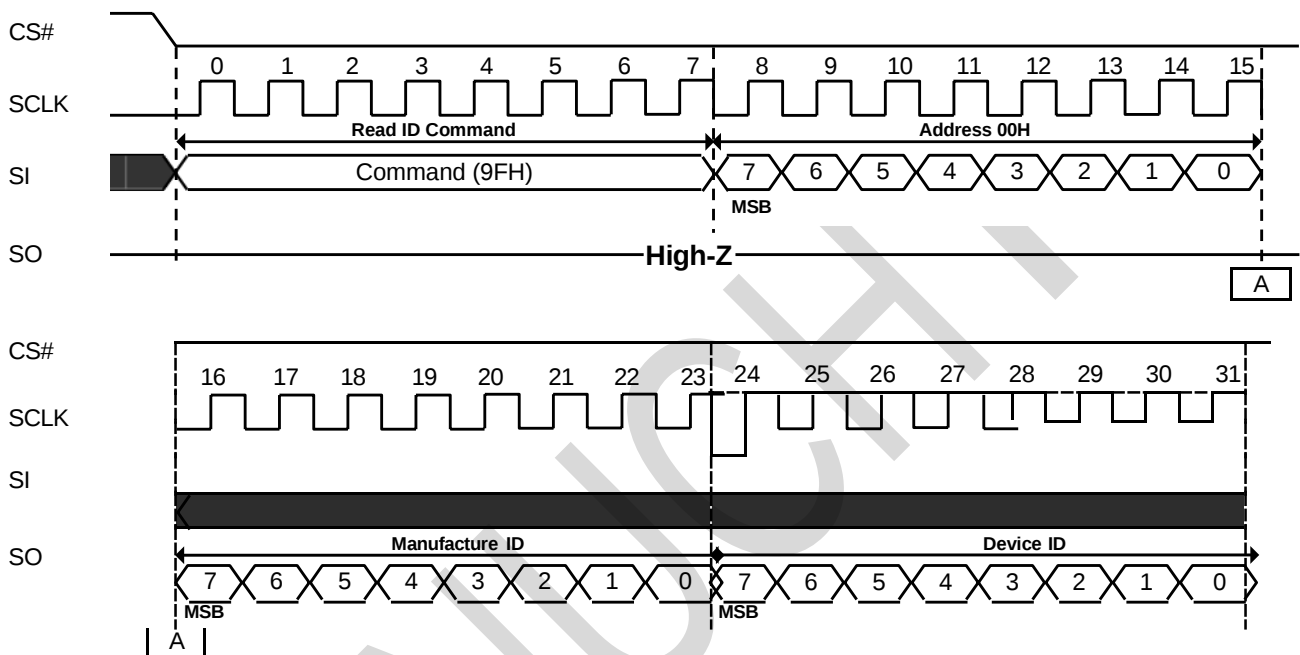
Figure 6-1. Read ID (9FH) Sequence Diagram
