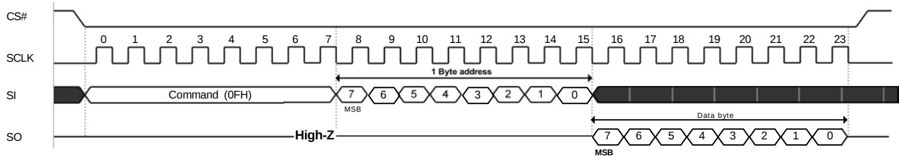
Figure 5-1. Get Feature (0FH) Sequence Diagram
