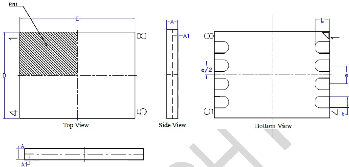
LGA-8 (8x 6 x 0.8mm)
