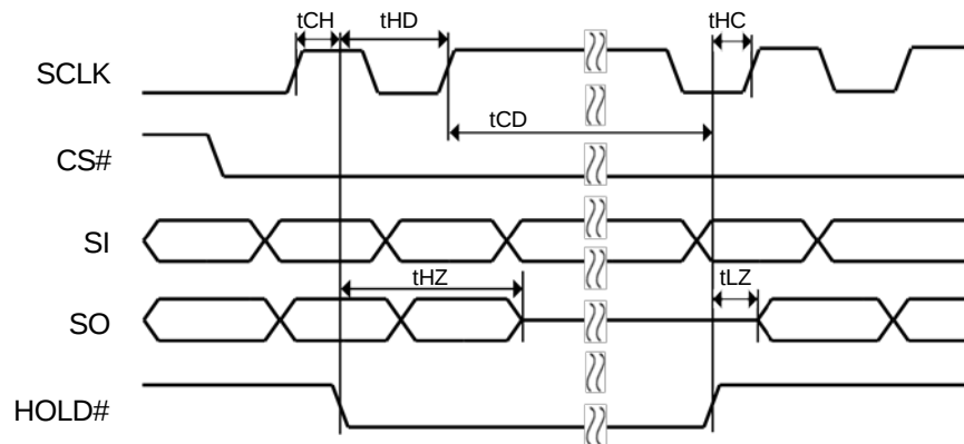
Figure 16-3. Hold# Timing
