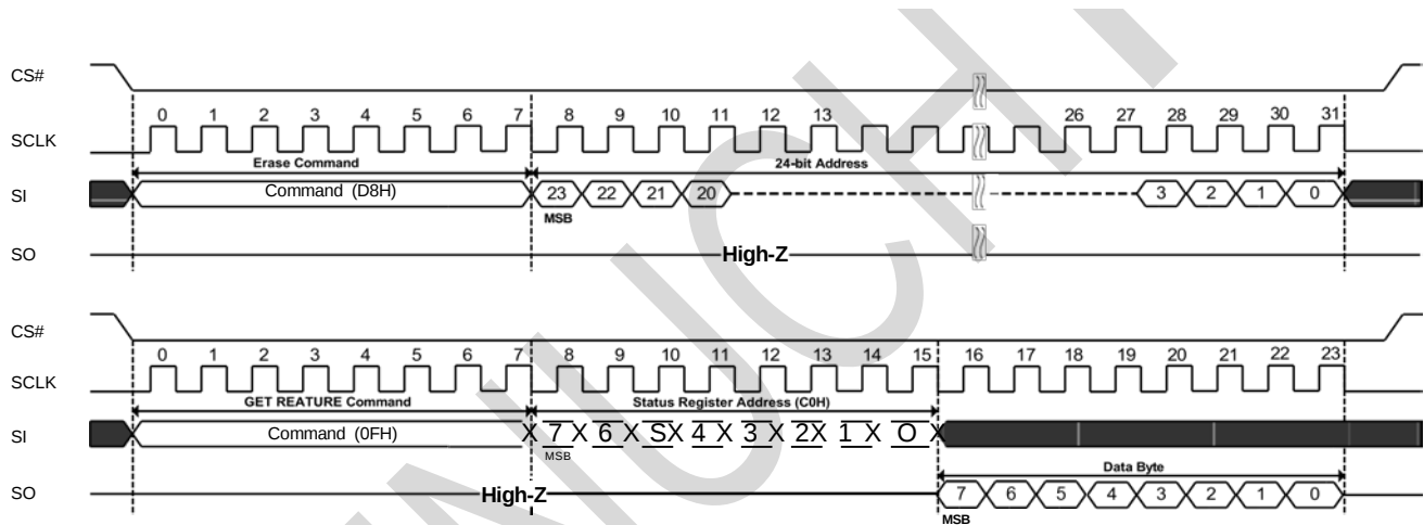
Figure 9-1. Block Erase (D8H) Sequence Diagram
