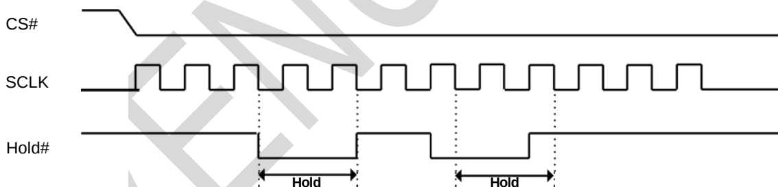
Figure 2-2. Hold Condition Diagram
