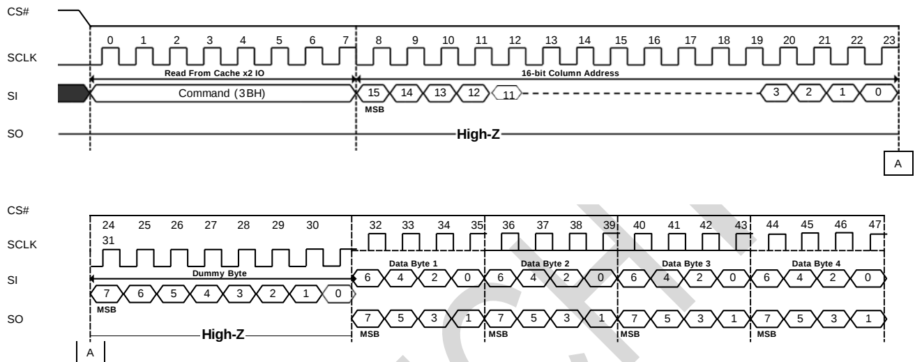
Figure 6-4. Read from Cache x2 IO (3BH) Sequence Diagram
