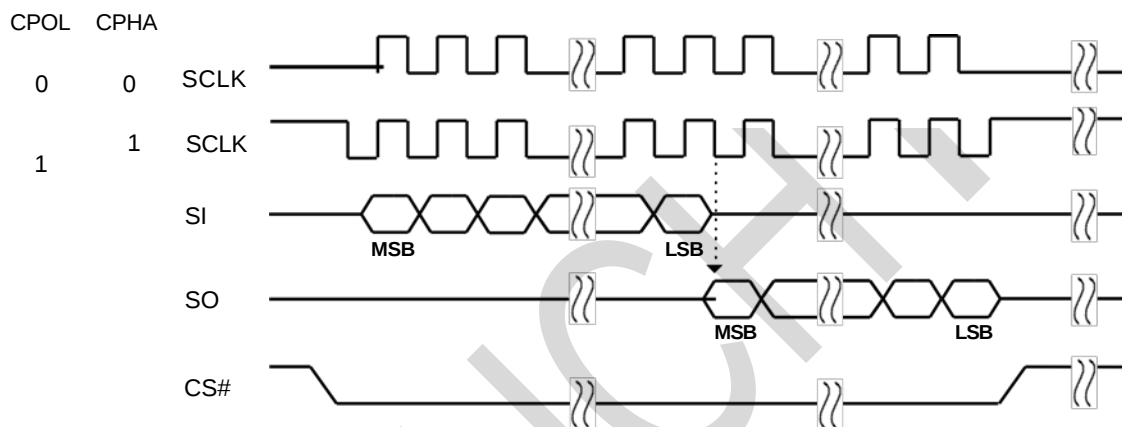
Figure 2-1. Timing Diagram of SPI Modes
