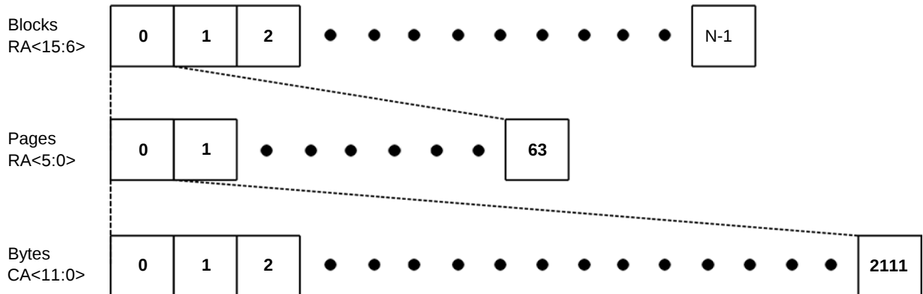
Figure 1-2. Memory Mapping Diagram for 2112 Page size
