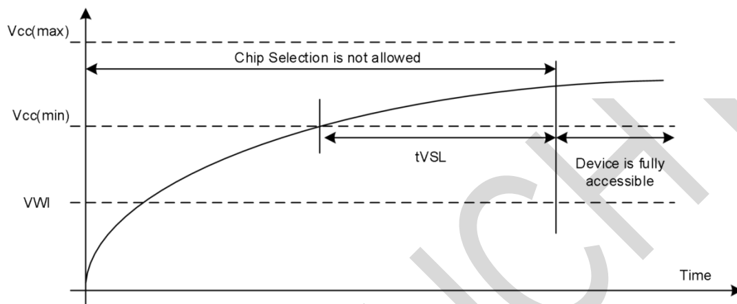
Figure15-1.Power on Timing Sequence
