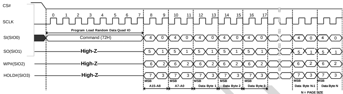
Figure 8-3. Program Load Random Data Quad IO (72H) Sequence Diagram
