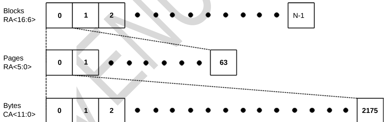
Figure 1-3. Memory Mapping Diagram for 2176 Page size
