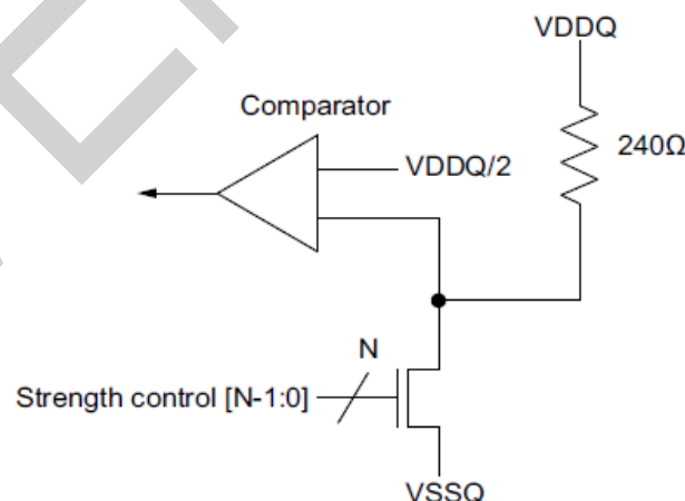
Figure 5-17 Pull-down Calibration
