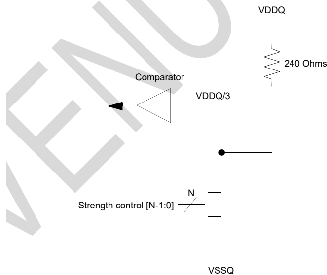
Figure 21. pull-down calibration
