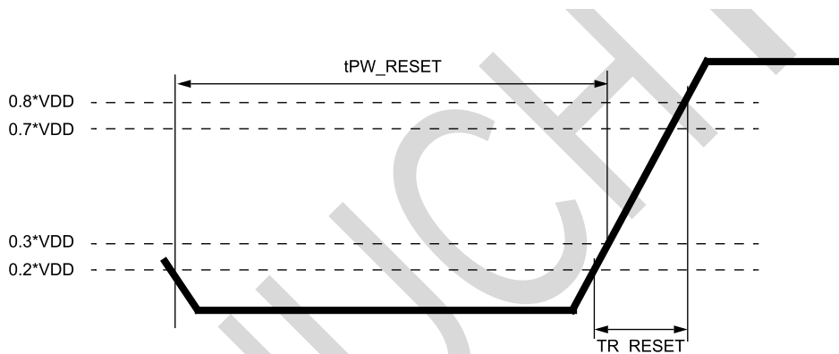
Figure 10. RESET n Input Slew Rate Definition
